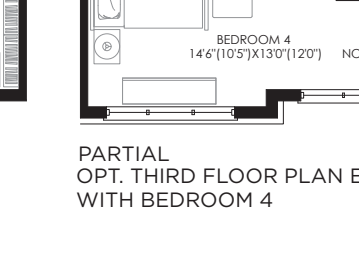
PARTIAL OPT. THIRD FLOOR PLAN ELEV. 'G' WITH BEDROOM 4
