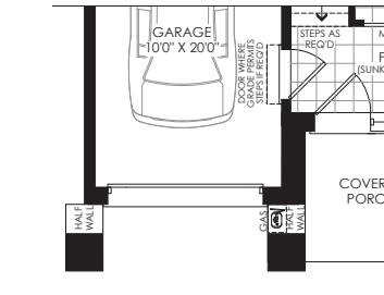
PARTIAL GROUND FLOOR PLAN ELEV. 'F'
